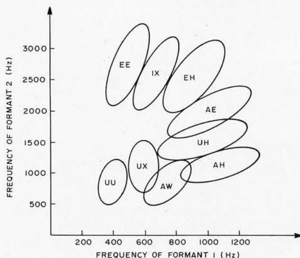
Figure 2: Vowel phonemes on the formant plane. "Formants" are the natural resonant frequencies of the vocal tract. These resonances are similar to the resonant vibrations of organ pipes or the characteristic sound of an empty bottle when air is blown across it. The three most prominent formants are centered around 500, 1500 and 2500 Hz, but they vary with changes in position of the tongue, lips and mouth.
